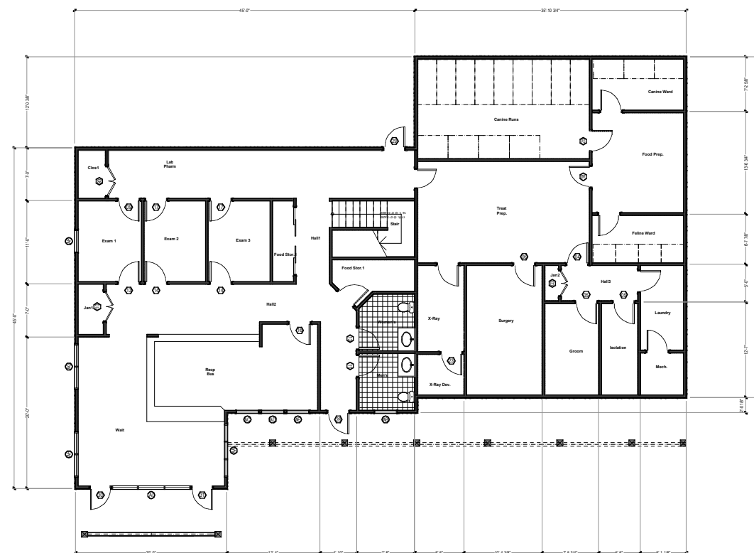
A Option A - Main Floor Plan 3,399.8 sq ft Gross area SK-2 Scale 1/4" = 1' - 0"
