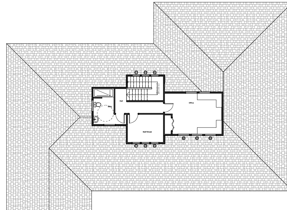
B Option A - Upper Floor Plan 600.3 sq ft Gross area SK-2 Scale 1/4" = 1' - 0"
